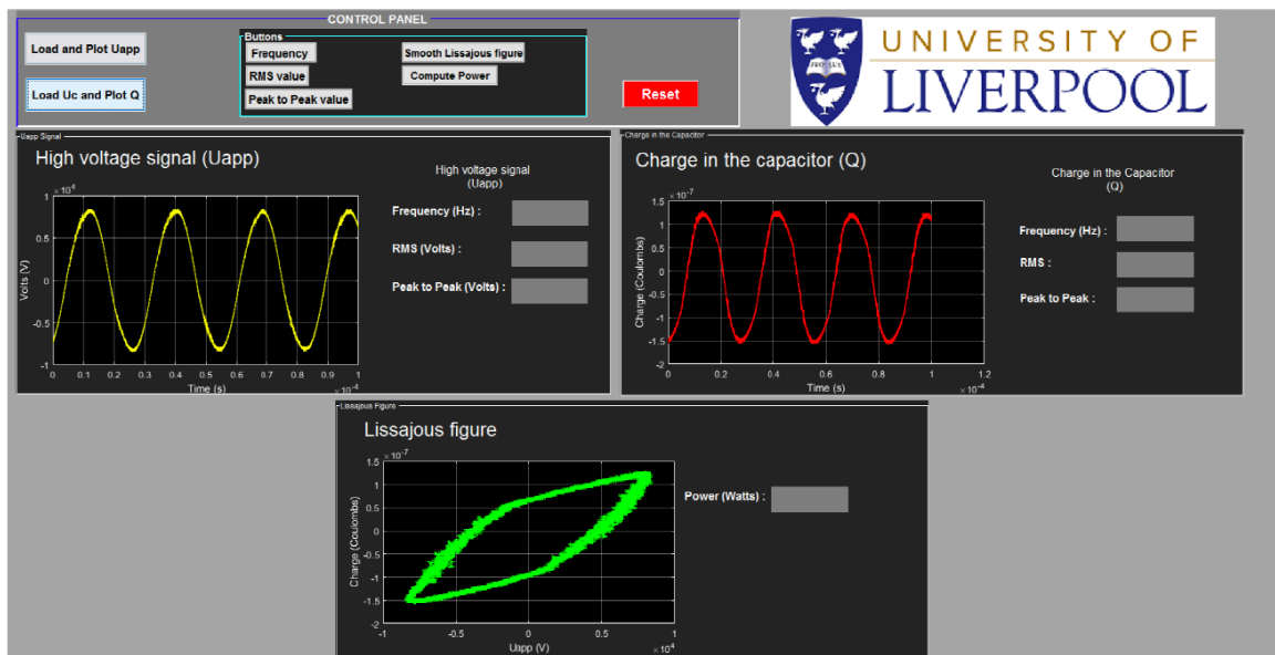
Figure 18: U_{app} , Q and Lissajous figure displayed in the interface
