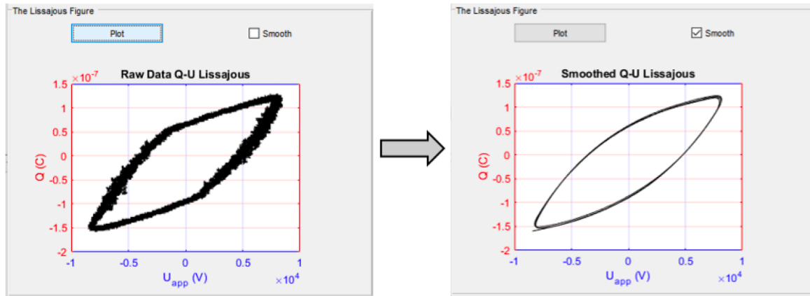
Figure 4: Plotting the raw-data Q-U Lissajous and implementing the smooth function.
