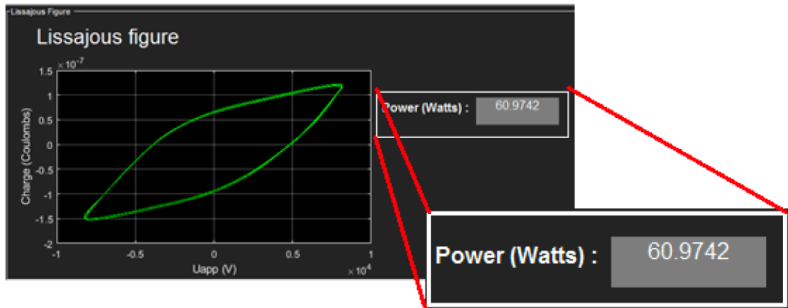
Figure 21: Value of the power in the GUI interface
