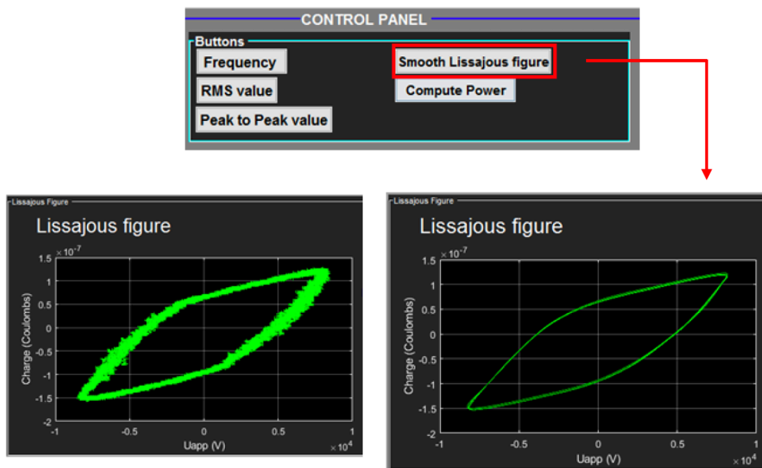
Figure 20: Smooth Lissajous Figure in the GUI interface
